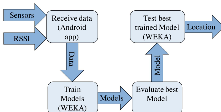
FIGURE 3.1: The architecture of the implemented android app.
