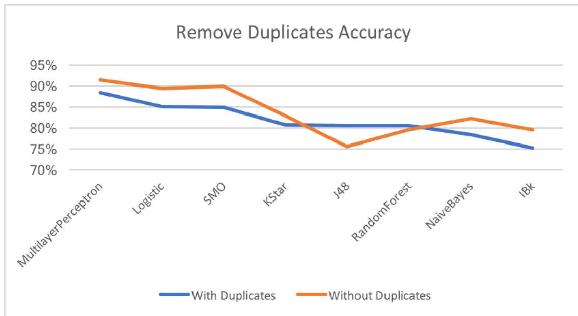
FIGURE 4.1: Landmark prediction accuracy with and without duplicate data points. Dataset Exeter Landmarks (see Section 3.5.2 and on https://github.com/JoelNiklaus/IndoLoc/tree/master/app/src/main/assets/thesis/exeter/landmark )
