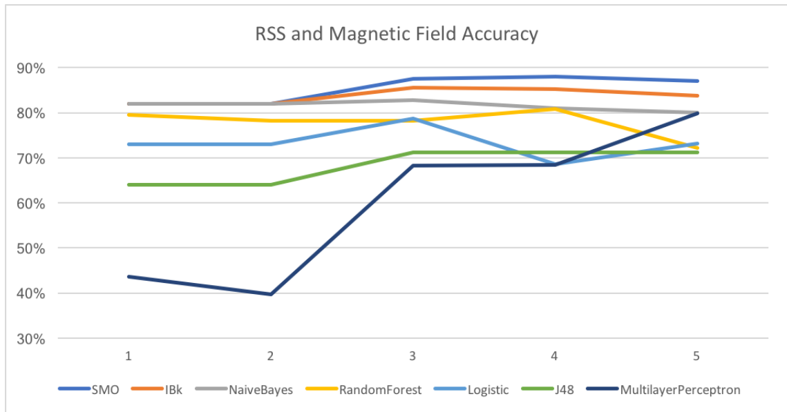
FIGURE 4.4: The accuracy with different ways of storing the magnetic field. Dataset Bern Rooms (see Section 3.5.1 and on https://github.com/JoelNiklaus/IndoLoc/tree/master/app/src/main/assets/thesis/bern/room ).
