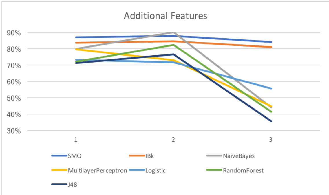
FIGURE 4.5: The accuracy with additional features added. Dataset Bern Rooms (see Section 3.5.1 and on https://github.com/JoelNiklaus/IndoLoc/tree/master/app/src/main/assets/thesis/bern/room ).
