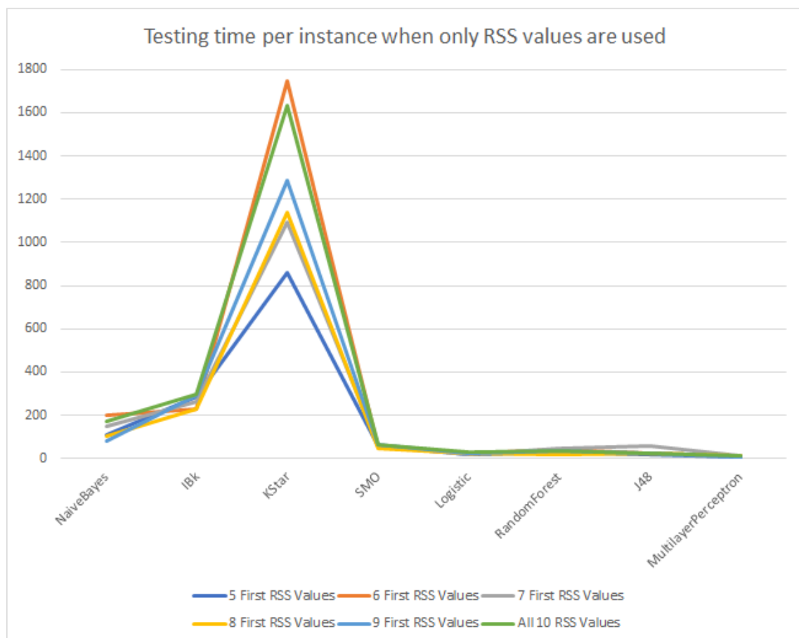
FIGURE 4.3: The testing time with a different number of RSS values measured in \mu s per instance. Dataset Bern Rooms (see Section 3.5.1 and on https://github.com/JoelNiklaus/IndoLoc/tree/master/app/src/main/assets/thesis/bern/room ).
