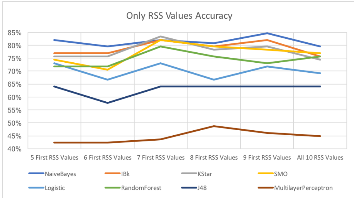
FIGURE 4.2: The accuracy with a different number of RSS values. Dataset Bern Rooms (see Section 3.5.1 and on https://github.com/JoelNiklaus/IndoLoc/tree/master/app/src/main/assets/thesis/bern/room )
